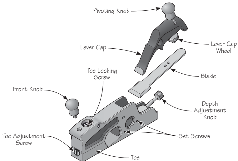
Figure 1: Large shoulder plane components.
